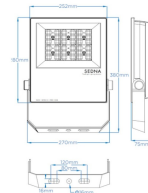
LED Premium Flood Light DIMENSIONS
